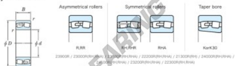
Boundary dimensions
