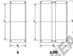
Backed needle roller and cage assemblies
