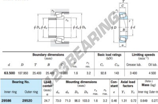
Single-row tapered roller bearings inch series Koyo
