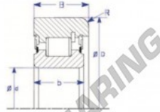
A One Piece IR, Snap Ring Style IV Roller Bearing
